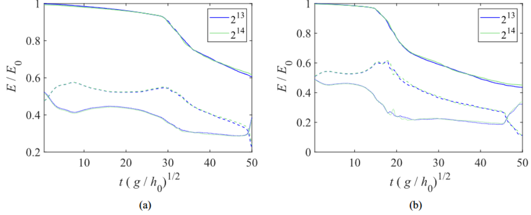
Figure 4.8 Comparison of energy budget between two mesh resolution levels 213 and 214 for two cases: (a) 0.2 initial wave amplitude, 2^\circ beach slope, and 0.3 storm surge depth; (b) 0.4 initial wave amplitude, 4^\circ beach slope, and 0.3 storm surge depth.
