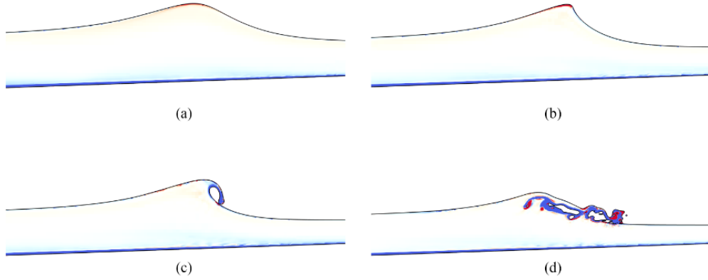
Figure B.1 Wave breaking process (plunging breaker) for the case with a beach slope of 2^\circ , an initial wave amplitude of 0.5, and a storm surge depth of -0.1 . Vorticity (color contour) in the water phase at the following four time instants: (a) t/t_0 = 13.2 , (b) t/t_0 = 15.6 , (c) t/t_0 = 17.2 , and (d) t/t_0 = 19.0 .
